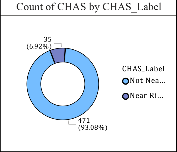
River vs Non-River Tract Split
